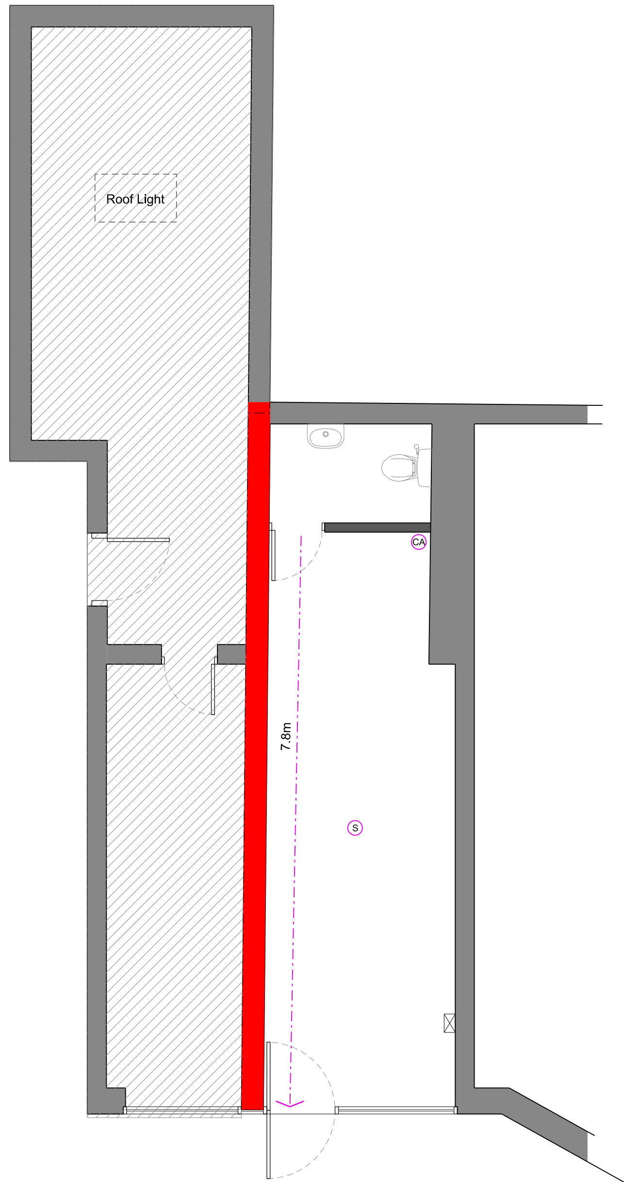
01 Fire Strategy Plan 50-0001 SCALE 1:50
